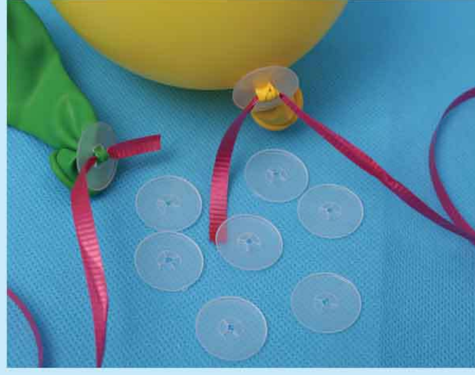
Item No.: LKBBA-008 Name: Round Pull buckle Size: 2X2cm Material: PP Packing: 1000/pcs Opp bag, 20000/pcs/CTN Meas: 52X33X34cm
